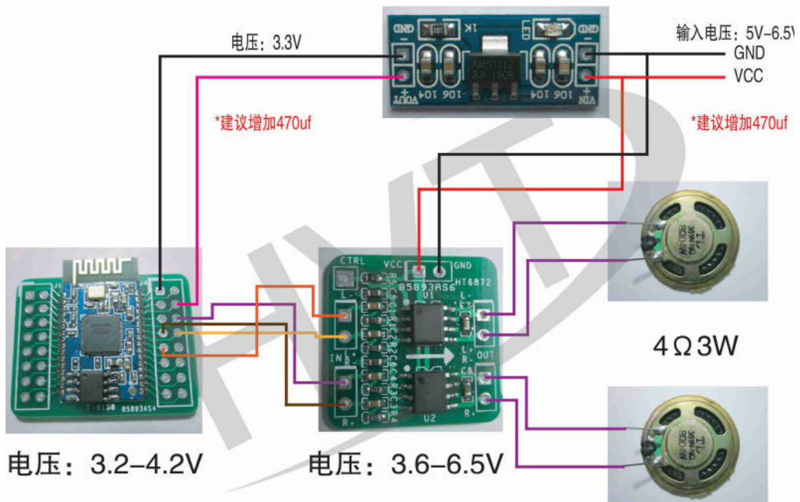
Based BK8000L simple Bluetooth headset SGM4812 --- 150mW (Differential-balanced) - Lithium battery power supply wiring
