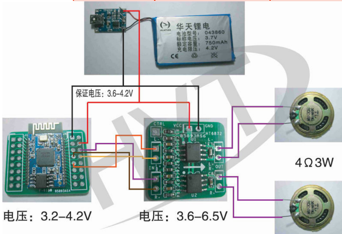
Based BK8000L simple Bluetooth stereo HT6872 --- 2x4Ω3W-5V power supply mode wiring diagram:
